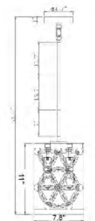
ZL32P7CH ZL32P7CO E12×3 Max40W
