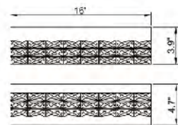
DIN08W16CH LED 8W (Include)
