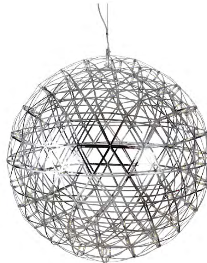
MN38SN(SATIN NICKEL) MN38GD(GOLD) SIZE:26"D LAMP:92/0.3W/LED 3000K MN37SN/MN37GD SIZE:18"D LAMP:42/0.3W/LED 3000K
