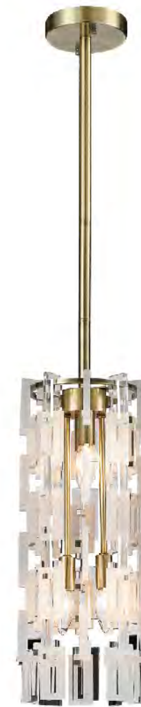
LX54P CL+FST SIZE:8"D×19"H LAMP:4/40W/E12 ACRYLIC LINK
