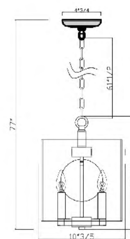
TG10GD TG10CH E12×4 Max40W
