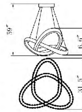
DIN03C31CH LED 52W (Include)
